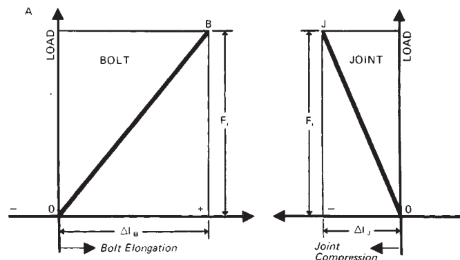
Fig. 1 (above) Joint components
