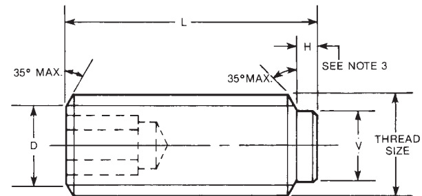
DOG POINT
